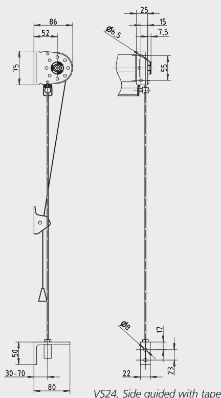
VS24, Side guided with tape
