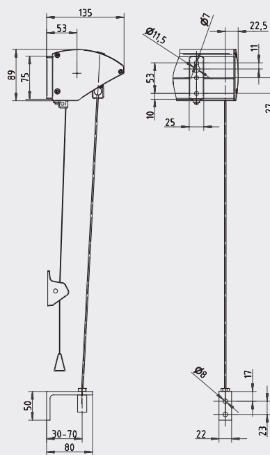
VS34, Side guided with tape
