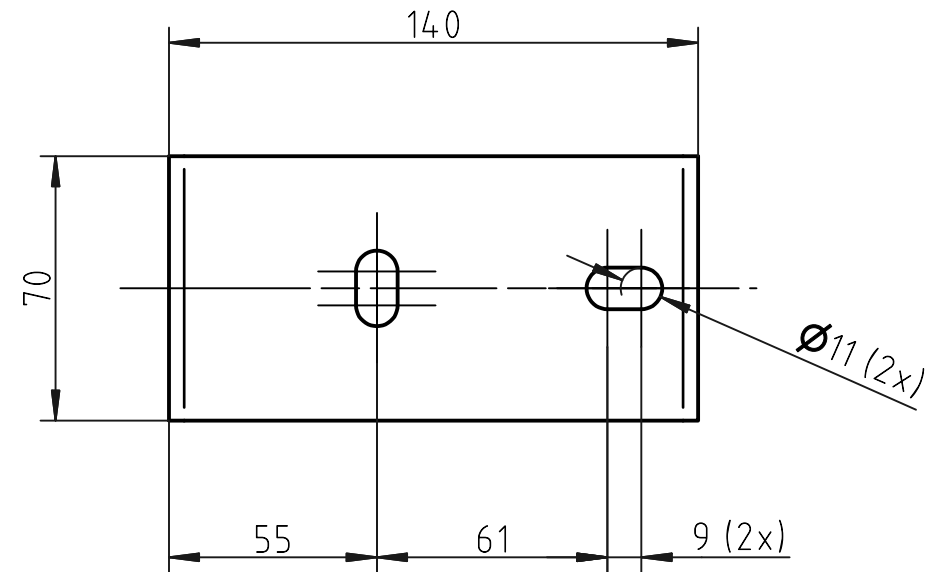
Roof bracket: (View A, from above)
